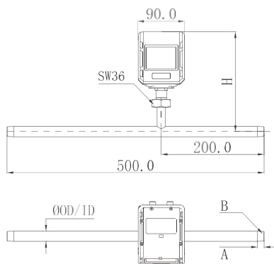
VC202x Thread-type dimension schematic
