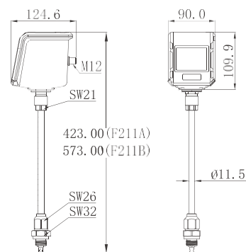
VC201x dimension schematic
